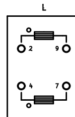
CommonModeChoke_WuerthType-WE-CMB_Size-L_RevA_25Oct2010
