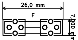
Fuseholder5x20_horiz_open_universal_Type - III_RevC_Date24Feb2011
