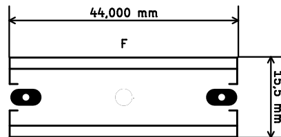
Fuseholder6x32_HorizontaL_Open_Schurter0031 - 8002_RevB_Date05Jul2010
