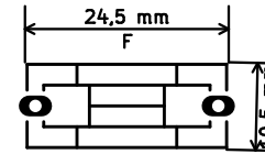
Fuseholder5x20_horiz_SemiClosed_Casing10x25mm_RevA_Date25Jul2010
