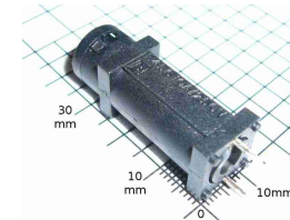
Fuseholder5x20_vert_closed_Bulgin_FX0456_RevB_Date05Jul2010
