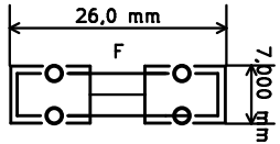
Fuseholder5x20_horiz_open_lateral_Type - I_L_RevC_Date24Feb2011
