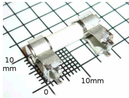
Fuseholder5x20_horiz_open_lateral_Type - I_L_RevC_Date24Feb2011
