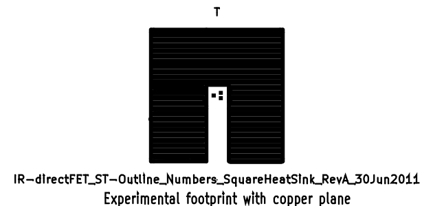
Heatsink Footprints of International Rectifiers directFet Transistor series.
