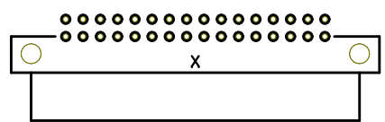
Socket_DIN41612_CaseB2_Male_32pin_2rows
