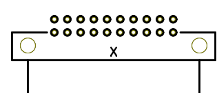
Socket_DIN41612_CaseB3_Male_20pin_2rows
