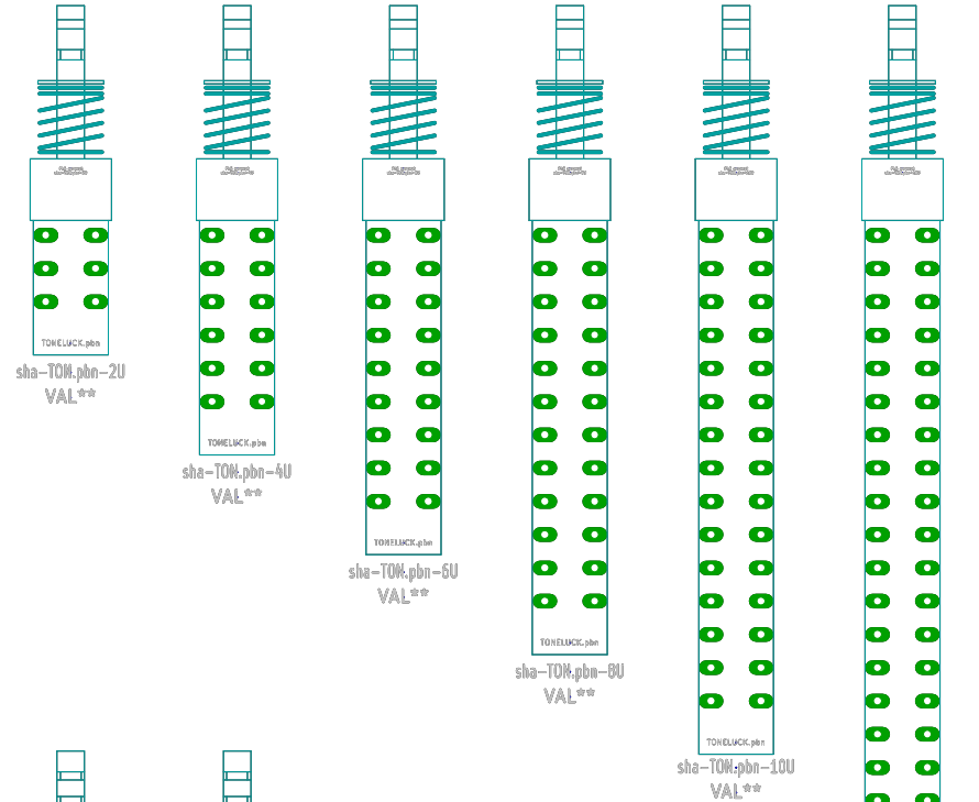
TONELUCK PBN series matrice 4mm x écartement 6mm
