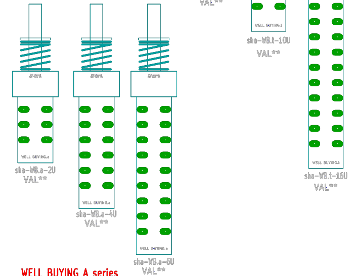
WELL BUYING A series matrice 4mm x écartement 6mm
