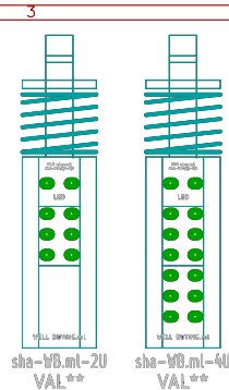
WELL BUYING ML series LED 3,7x3 matrice 2,5mm x écartement 3mm
